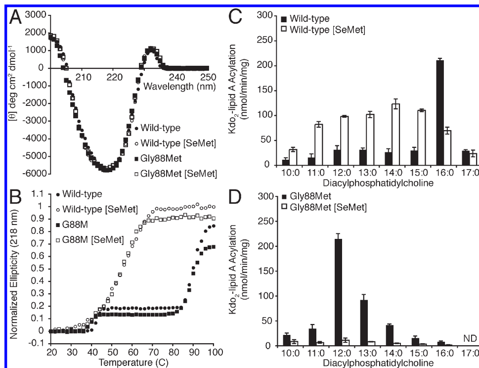
FIGURE 6: SeM substitution is highly destabilizing to PagP. Far-UV CD (A) and thermal melts at 218 nm (B) reveal that substituting methionines in wild-type and Gly88Met PagP with SeM compromises stability. PagP specific activity was measured using defined PtdCho's varying in saturated acyl chain length from C17 to C10. Wild-type (C) and Gly88Met (D) PagP were monitored with and without SeM substitution. ND means not detected.
