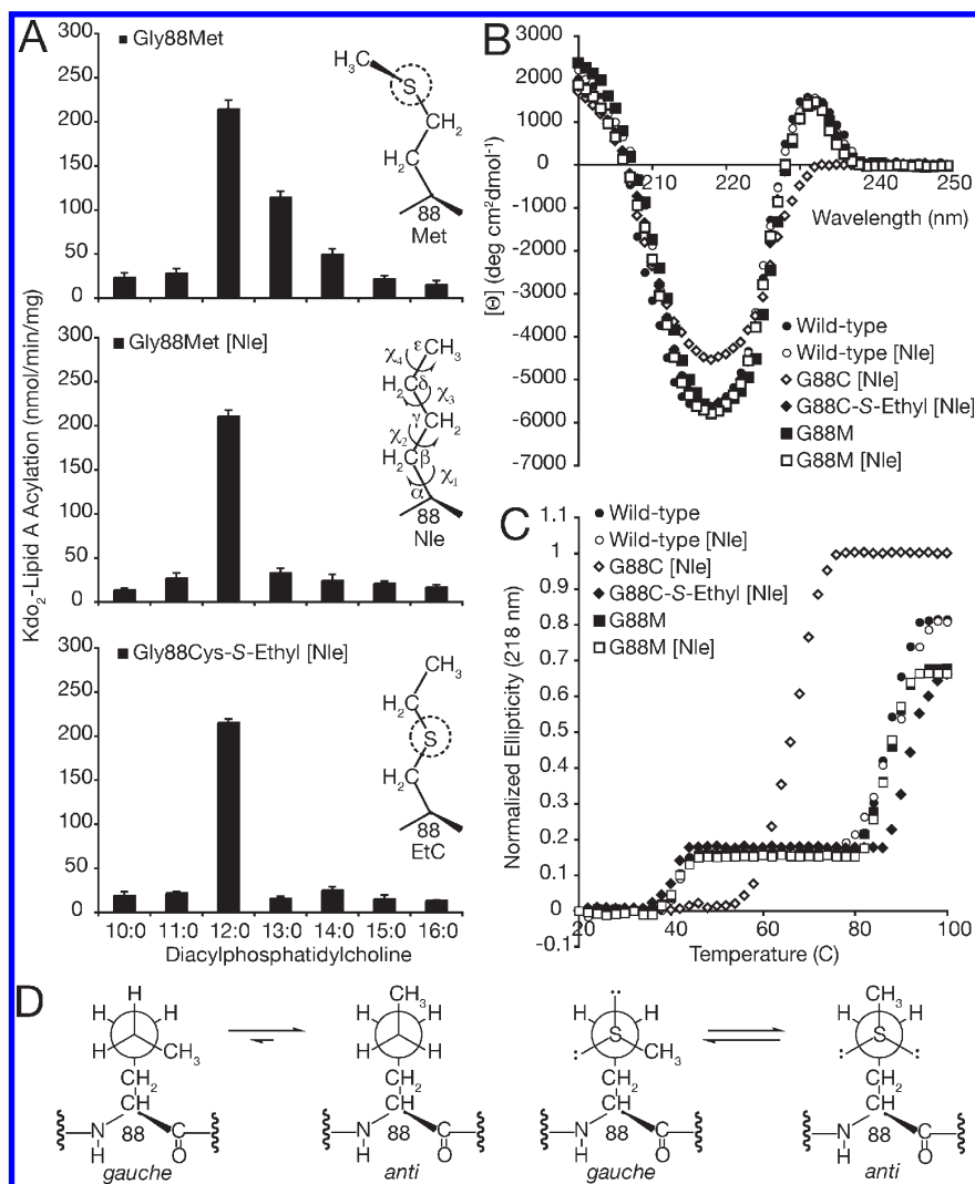
FIGURE 4: Role of side chain flexibility and localized thioether–aromatic dispersion attraction in engineering a dedicated PagP lauroyltransferase. (A) PagP specific activity was measured using defined PtdCho's varying in saturated acyl chain length from C16 to C10. The unnatural amino acid Nle was substituted for Met by misaminoacylation of tRNA Met . Panels from top to bottom represent the activity profiles for Gly88Met, Gly88Met [Nle], and Gly88Cys-S-ethyl [Nle], respectively. For comparison, the behavior of Gly88Cys-S-ethyl PagP is shown in Figure 2. (B) Far-UV CD and (C) thermal melts at 218 nm reveal that substituting the five methionines in wild-type and Gly88Cys PagP (six in Gly88Met PagP) with Nle does not compromise structure or stability. (D) Schematic representation of side chain conformational preferences for Nle (left) and Met (right). Viewed in Newman projection down the central \chi_3 torsion axis, the penultimate atom is rotated to emphasize the enthalpic preference of Nle for maintaining the terminal methyl group in the extended anti conformation, whereas Met is slightly favored to adopt one of the two available gauche conformers.
